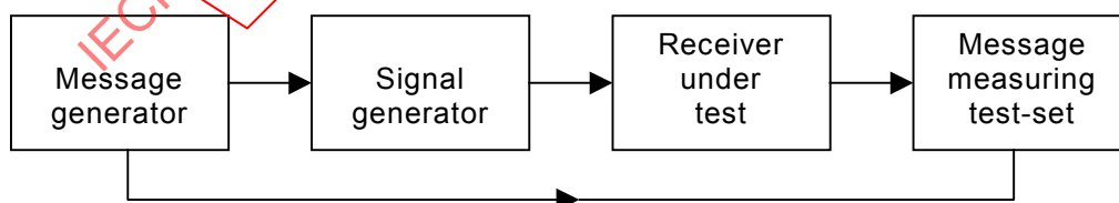
Figure 7 – Measurement arrangement
