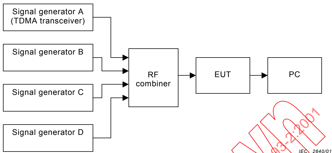
Figure 12 – Test set-up
