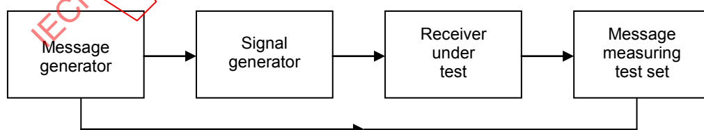
Figure 8 – Measurement arrangement
