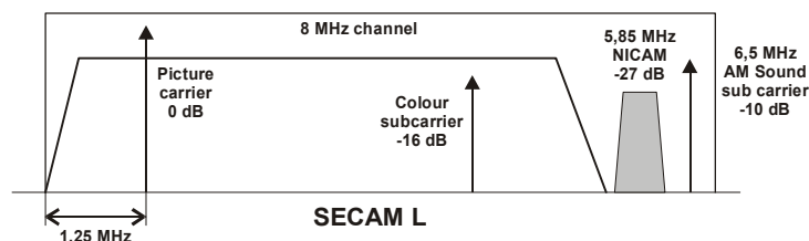
Figure 6 – SECAM L interfering signal
