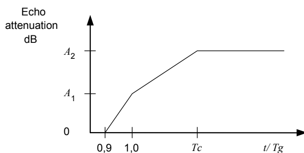
Figure 12 – Echo outside guard interval mask
