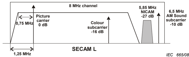
Figure 10 – SECAM L interfering signal
