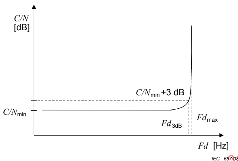
Figure 5 – DVB-H reference receiver C/N behaviour in mobile channel
