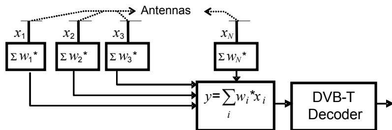
Figure 3 – Antenna diversity receiver
