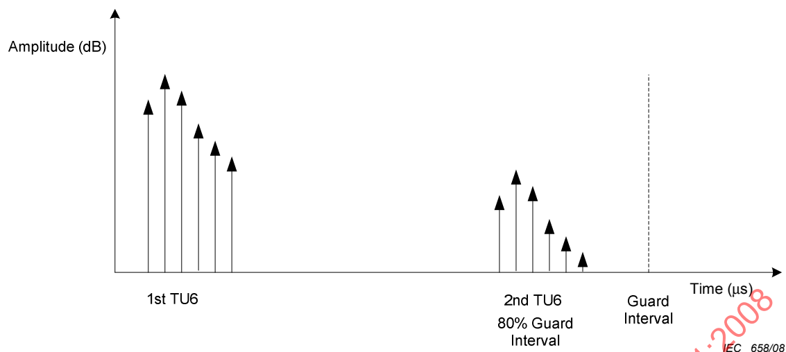
Figure 6 – Mobile SFN synchronisation test channel for weak long echo
