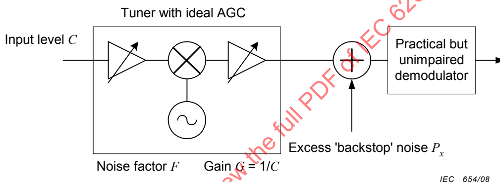
Figure 2 – Noise model
