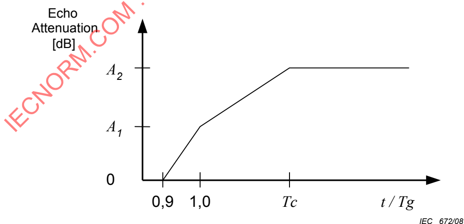
Figure 17 – Echo outside guard interval mask
