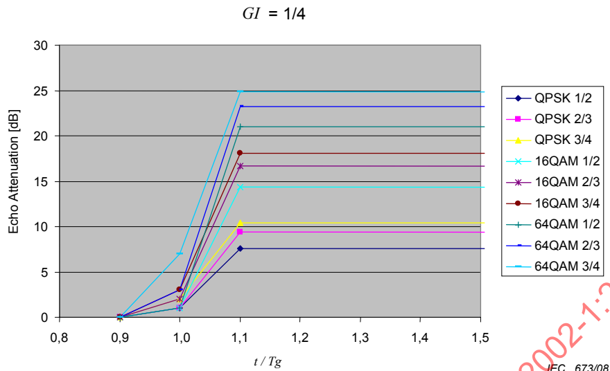
Figure 18 – Mask for echo outside GI for GI = 1/4
