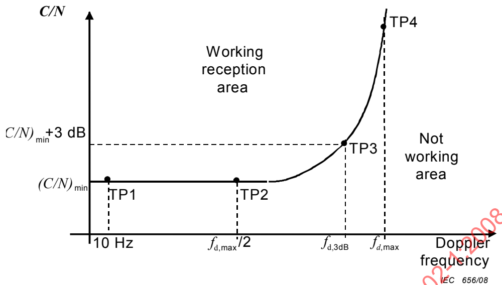
Figure 4 – Receiver behaviour in a mobile channel
