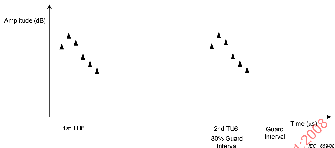
Figure 7 – Mobile SFN synchronisation test channel for strong long echo
