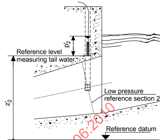
Figure B.3 – Measuring section at draft tube
