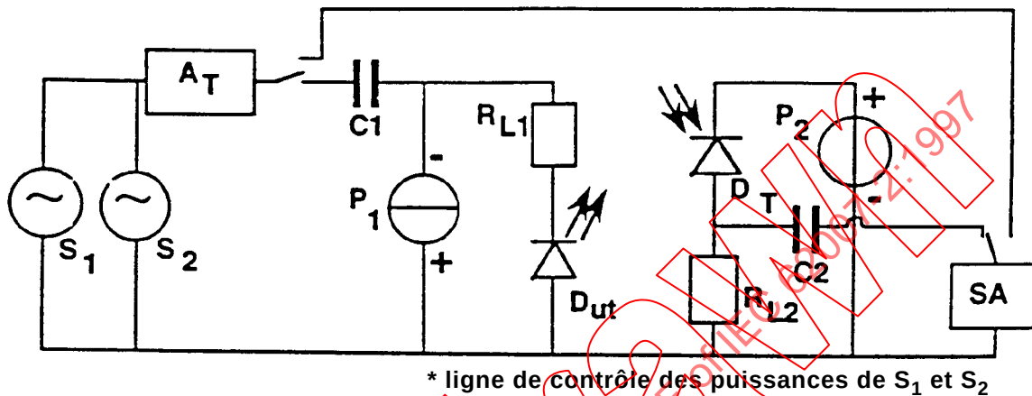
Figure 25 – Schéma
