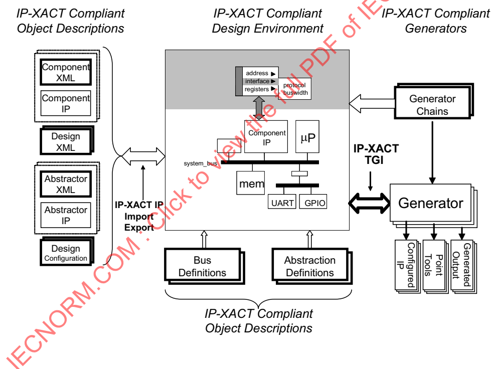
Figure 1—IP-XACT design environment
