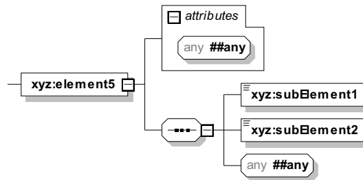
Figure 7—Wildcards
