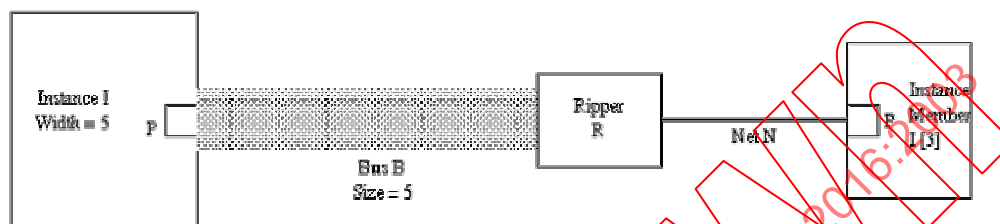
Figure 20 – Connectivity ripper
