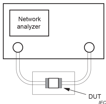
Figure 11 – Schematic diagram of the two-port S-parameter measurement setup and the network analyzer
