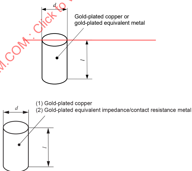
Figure 6 – Short device shape
