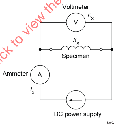
Figure 3 – Temperature rise measurement measuring circuit by resistance substitution method
