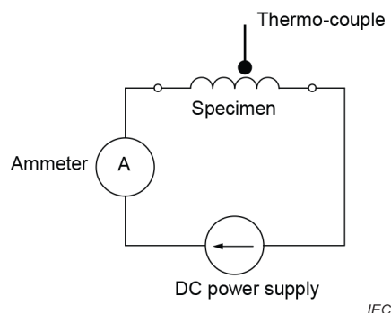
Figure 4 – Temperature rise measurement measuring circuit by thermo-couple method
