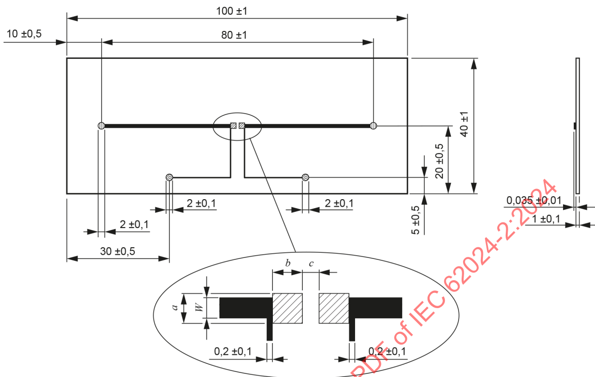
a) Example of printed-wiring board for SMD type ( I_{\text{class A}} )
