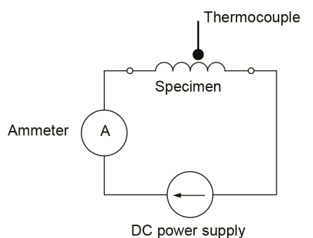
Figure 4 – Temperature rise measuring circuit by thermocouple method
