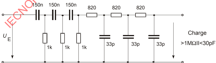
Figure 73 – Passe-bande (10 kHz ... 500 kHz)
