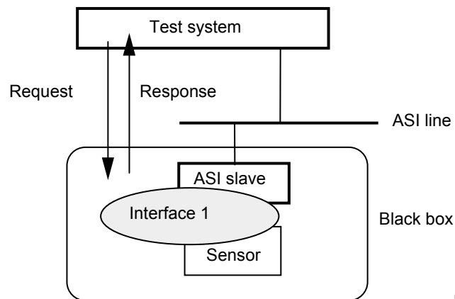
Figure 59 – AS-i interfaces
