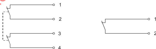
Figure A.7 – Connection of mechanical switches
