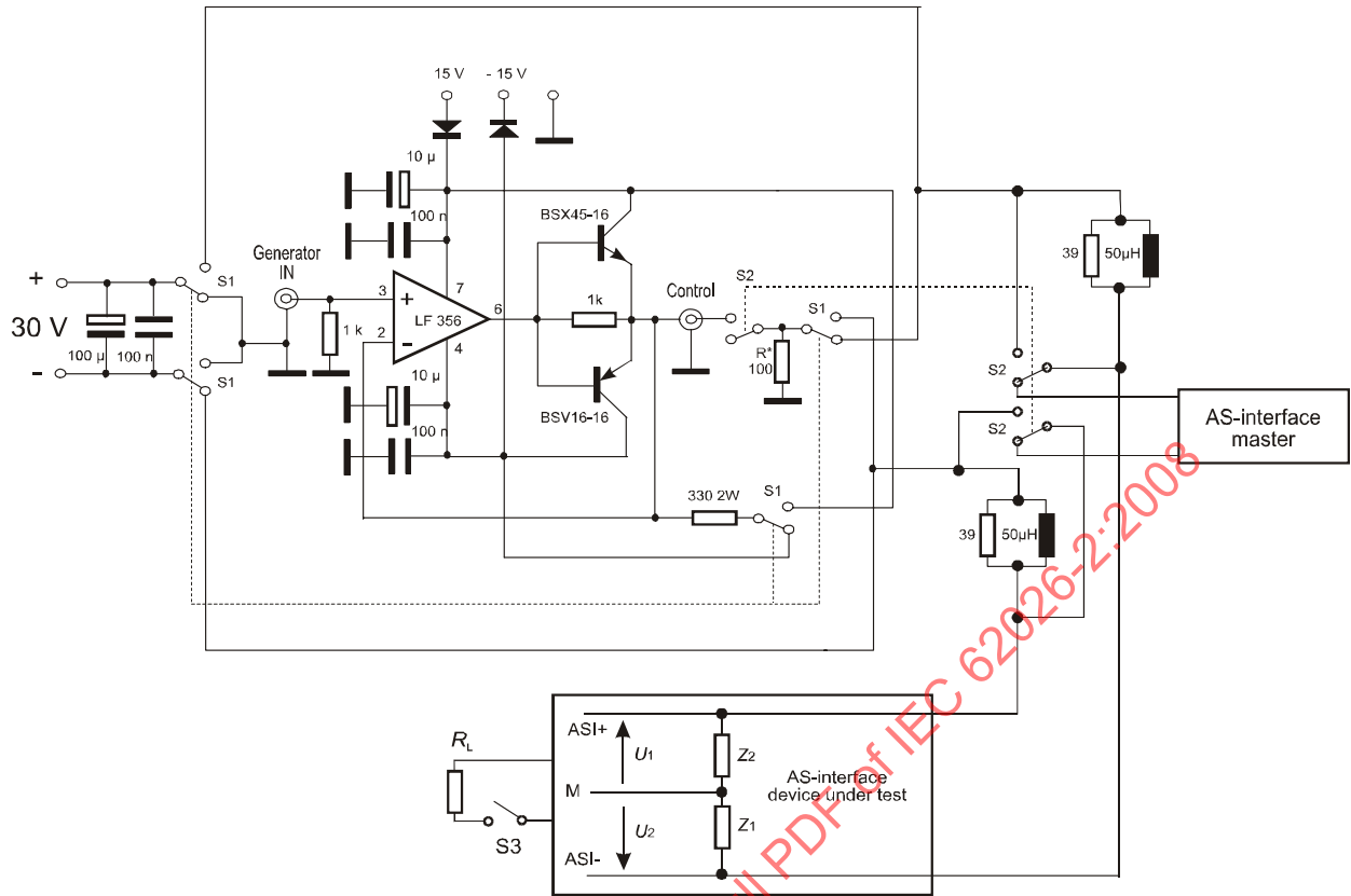
Figure 87 – Test circuit
