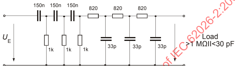
Figure 102 – Bandpass 10 kHz to 500 kHz
