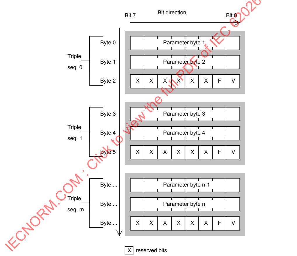
Figure A.5 – Data structure of the parameter string (S-7.4)
