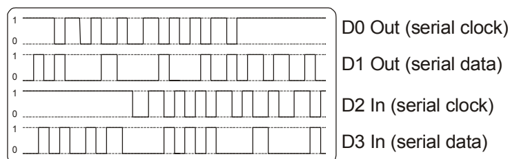
Figure 42 – Typical combined transaction type 2 signals (the master transmits the byte 10101011_{\text{Bin}} , the slave transmits 01110101_{\text{Bin}} ):
