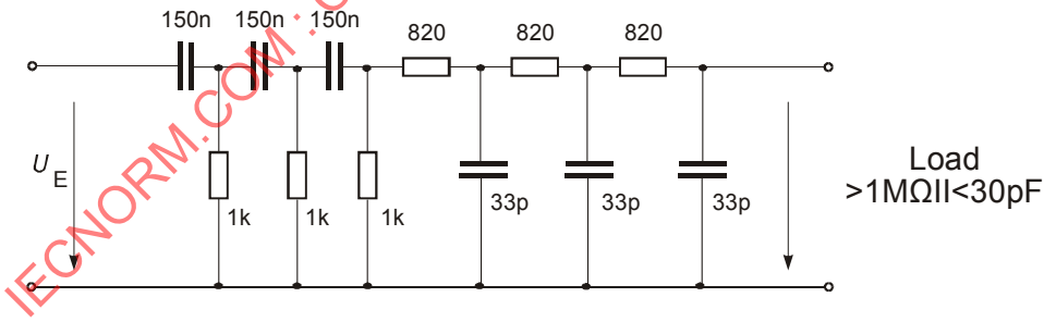
Figure 73 – Bandpass (10 kHz ... 500 kHz)
