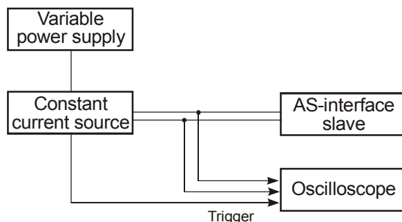
Figure 84 – Test circuit
