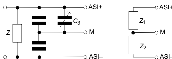
Figure 53 – A slave with C3 to compensate for Z_1 = Z_2
