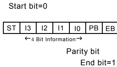
Figure 11 – Structure of a slave response
