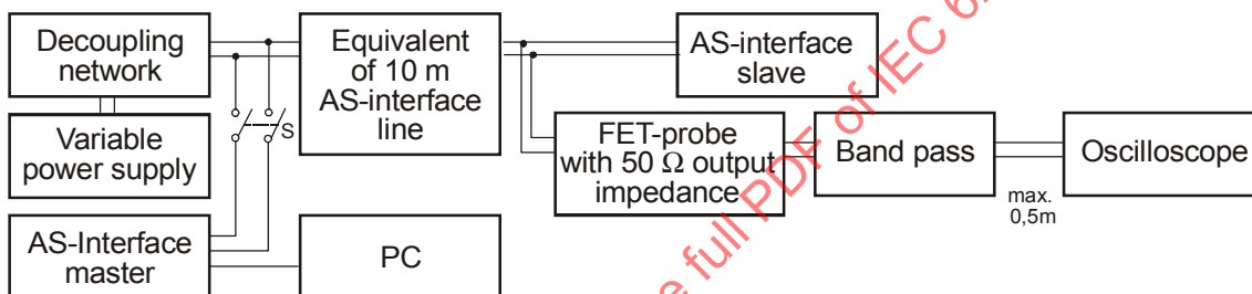
Figure 80 – Test circuit
