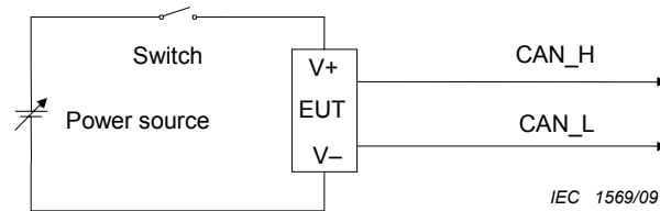
Figure 65 – Power ON test circuit
