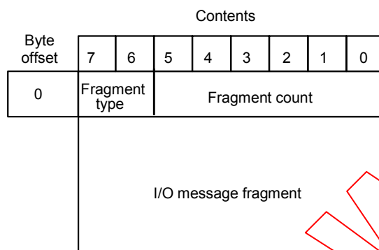
Figure 18 – I/O message fragment format
