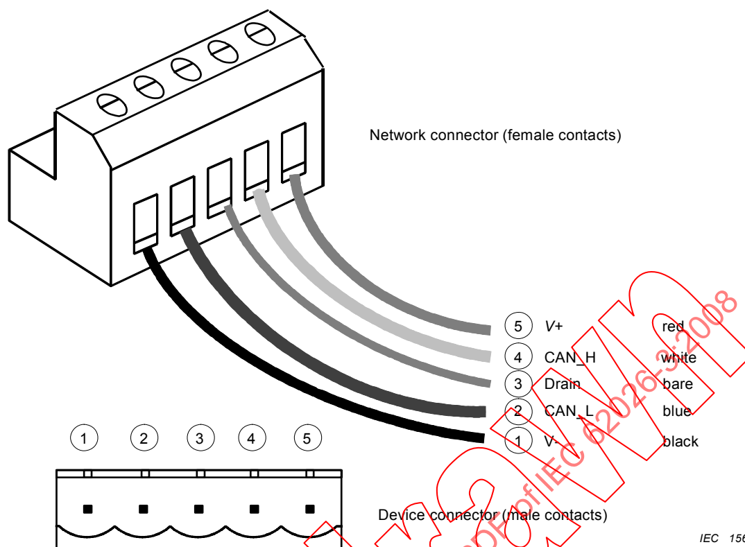
Figure 57 – Open connector pinout
