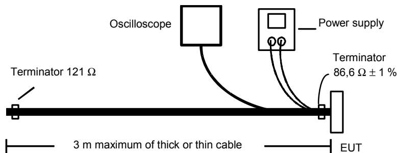
Figure 68 – Transmit level test setup
