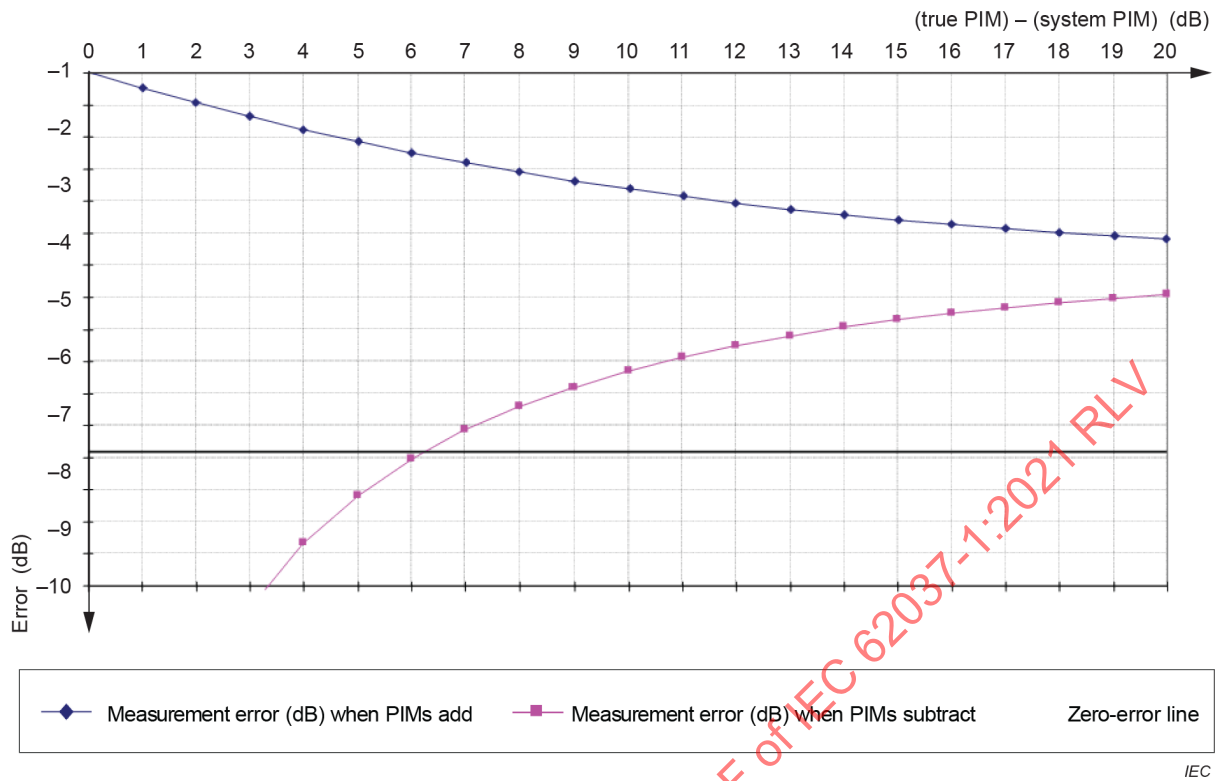
Figure 3 – Passive intermodulation (PIM) measurement error caused by residual system error
