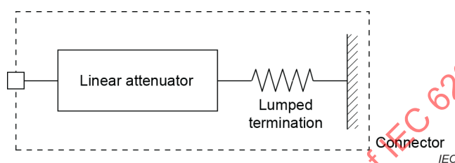
Figure A.2 – Lumped termination with a linear attenuator
