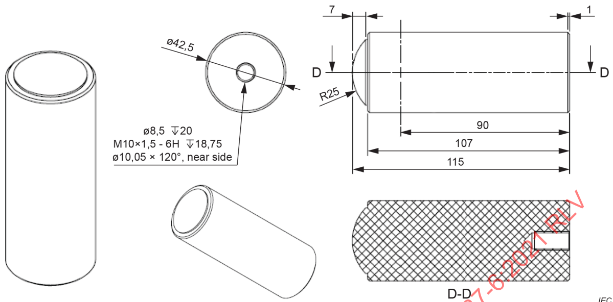
Figure 3 – Hammer description
