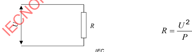
Figure BB.1 – Reference resistive load
