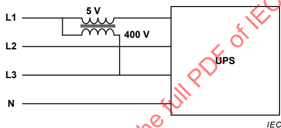
Figure D.2 – Phase unbalance
