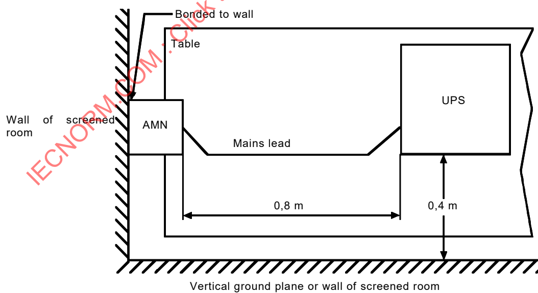
Figure A.8 – Test configuration for table-top equipment (conducted emission measurement) – Plan view
