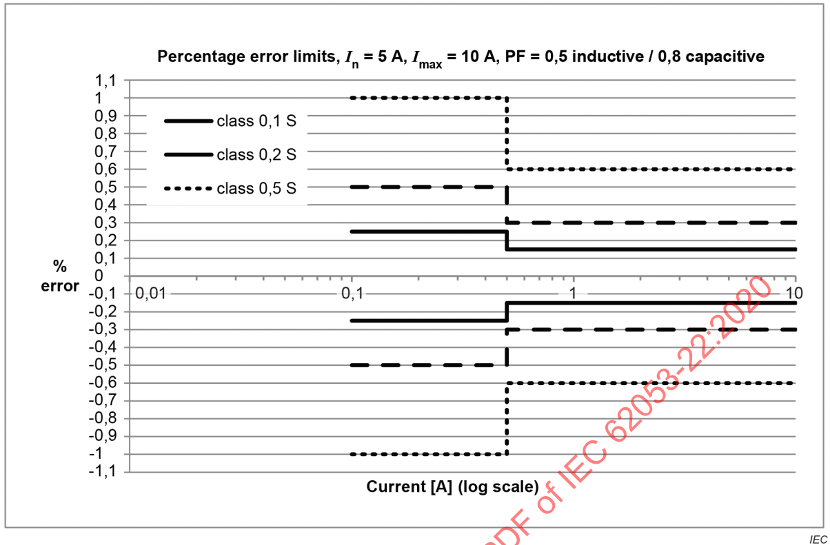
Figure A.2 – Comparison of acceptable percentage error limits for meters of classes 0,1 S, 0,2 S, and 0,5 S with I_n = 5\text{ A} and I_{\max} = 10\text{ A} , at PF = 0,5 inductive or PF = 0,8 capacitive
