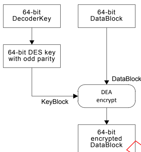
Figure 19 – DEA: EncryptionAlgorithm09
