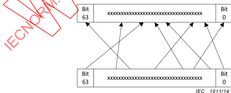
Figure 23 – STA decryption permutation process
