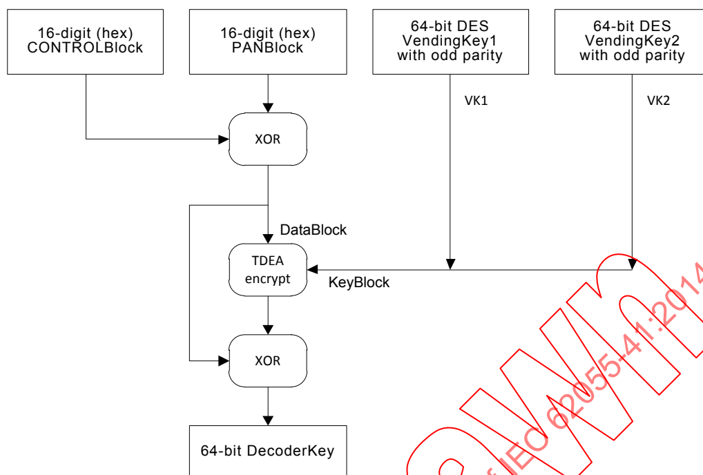
Figure 13 – DecoderKeyGenerationAlgorithm03
