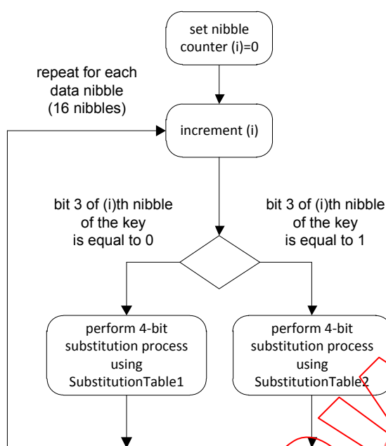
Figure 15 – STA encryption substitution process
