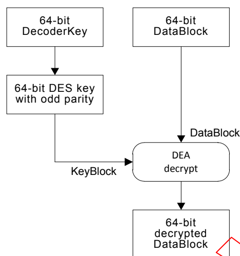
Figure 27 – DEA DecryptionAlgorithm09
