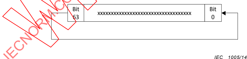
Figure 17 – STA encryption DecoderKey rotation process
