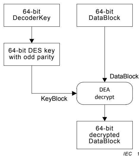
Figure 27 – DEA Decryption Algorithm
