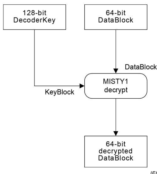
Figure 26 – STA DecryptionAlgorithm11
