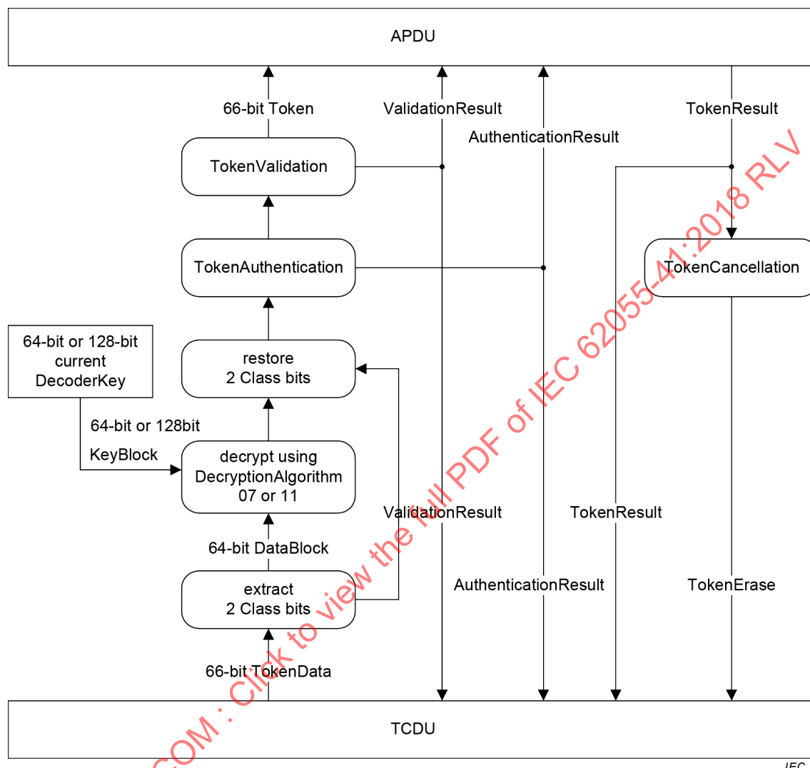
Figure 19 – APDUExtraction function
