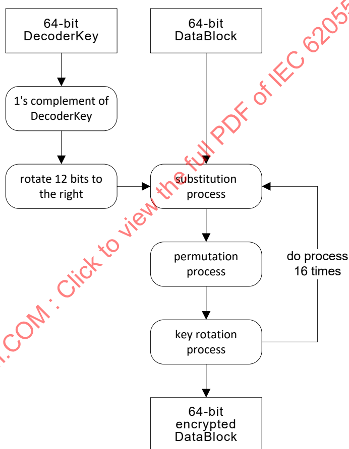
Figure 12 – STA: EncryptionAlgorithm07
