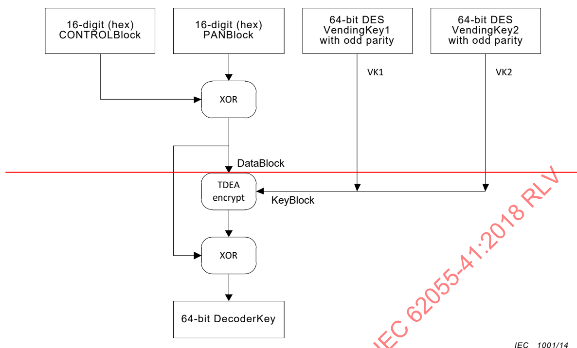
Figure 13 – DecoderKeyGenerationAlgorithm03
