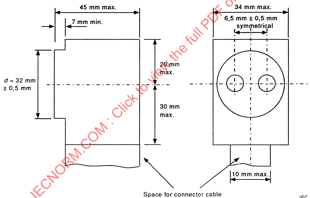
Figure 2b – Dimensions
