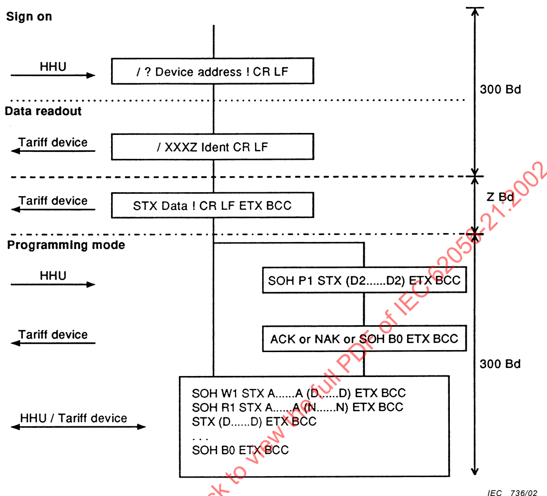
Figure 10 – Diagram protocol mode B
