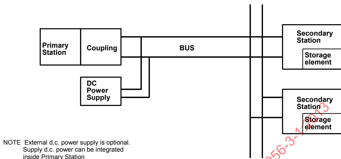
Figure 7 – Bus representation
