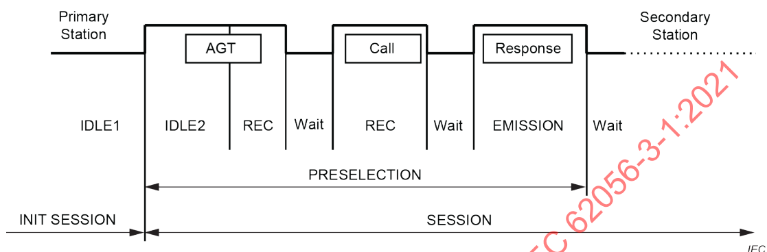
Figure 9 – States associated to a session: for selected Secondary Station
