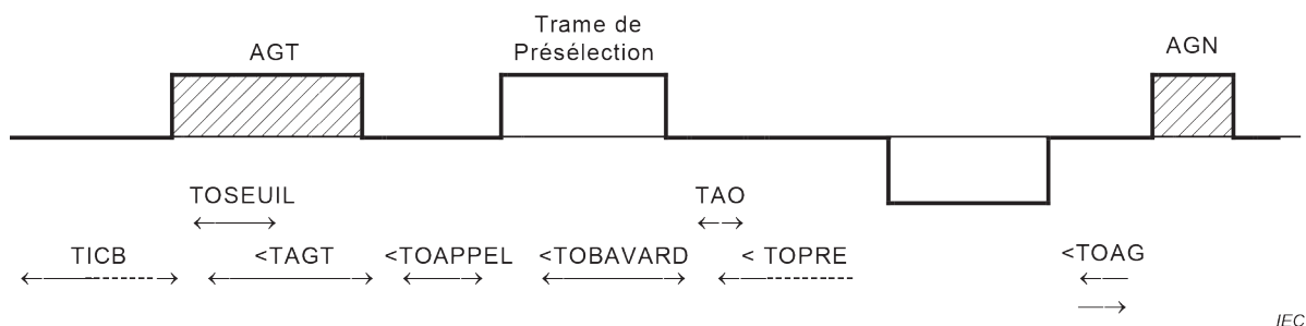
Figure 3 – Échanges sans interruption
