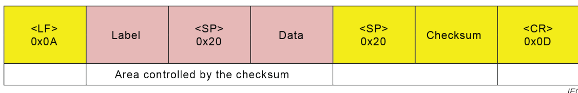
Figure 17 – Historical TIC: information group structure
