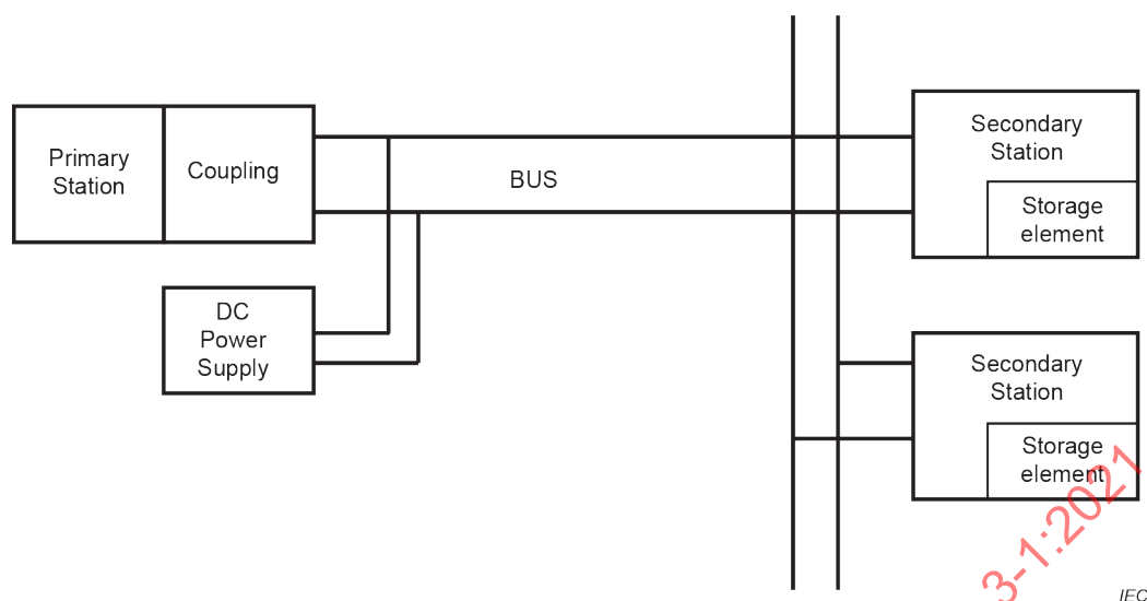
Figure 7 – Bus representation
