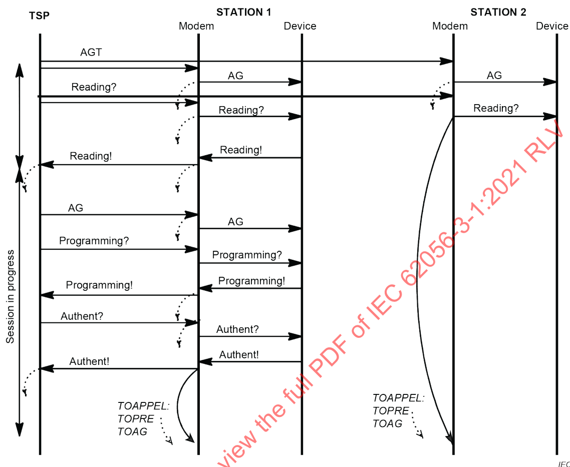
Figure I.2 – Remote reading and programming exchanges
