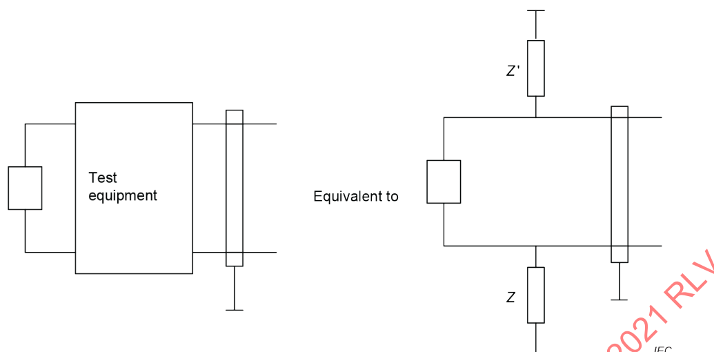
Figure 20 – Equivalent diagram of the test equipment
