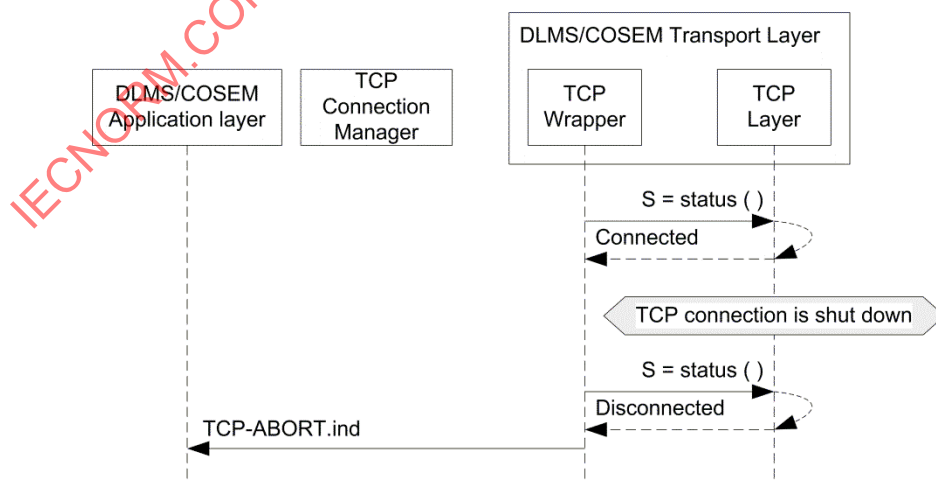
Figure A.4 – Polling the TCP sublayer for TCP abort indication
