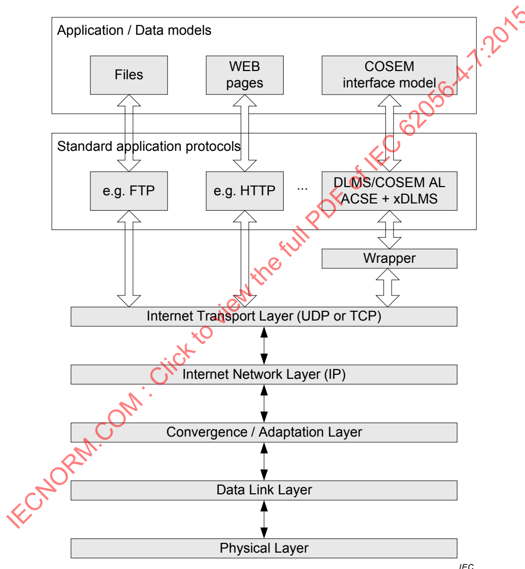
Figure 1 – DLMS/COSEM as a standard Internet application protocol
