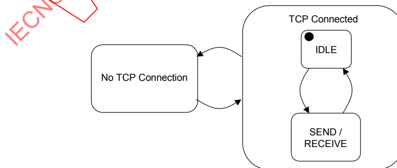
Figure 11 – High-level state transition diagram for the wrapper sub-layer
