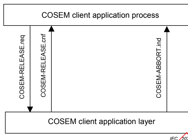
Figure 10 – Client side services for releasing an application association
