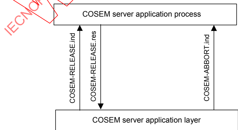
Figure 14 – Server side services for releasing an application association
