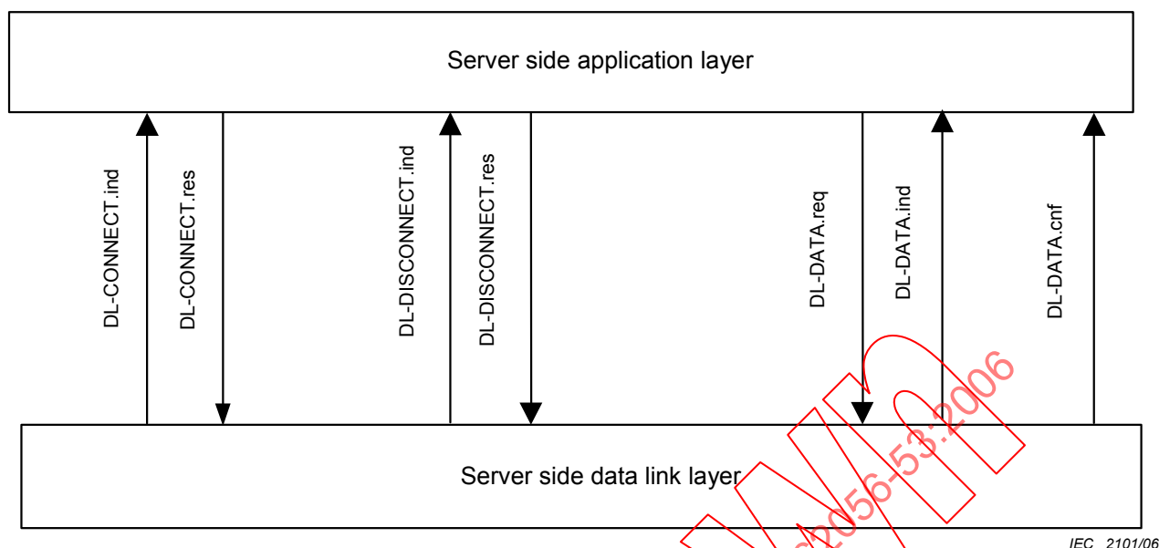
Figure B.3 – Data link layer services provided to and used by the server COSEM application layer
