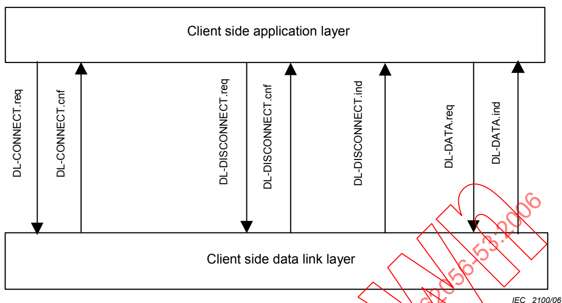
Figure B.2 – Data link layer services provided to and used by the client COSEM application layer
