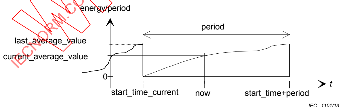
Figure 7 – The attributes in the case of block demand
