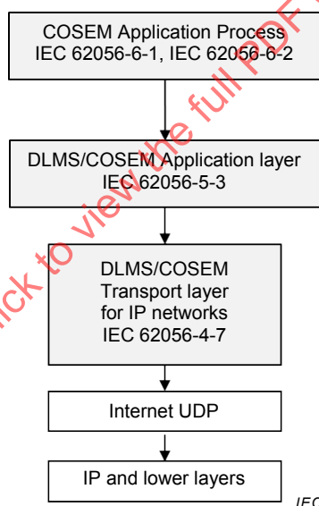
Figure E.1 – Structure of the IP profile
