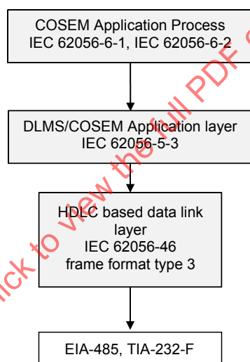
Figure C.1 – Structure of the RS485/232 profile
