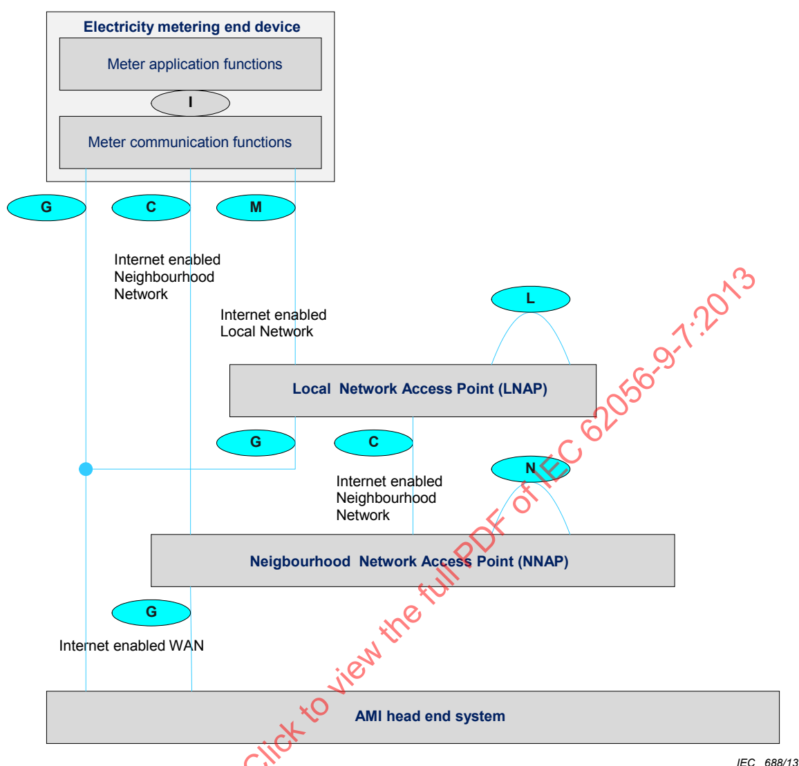
Figure 1 – Communication architecture
