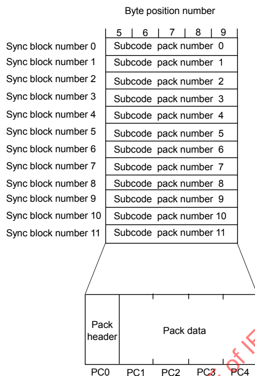
Figure 36 – Arrangement of subcode data
