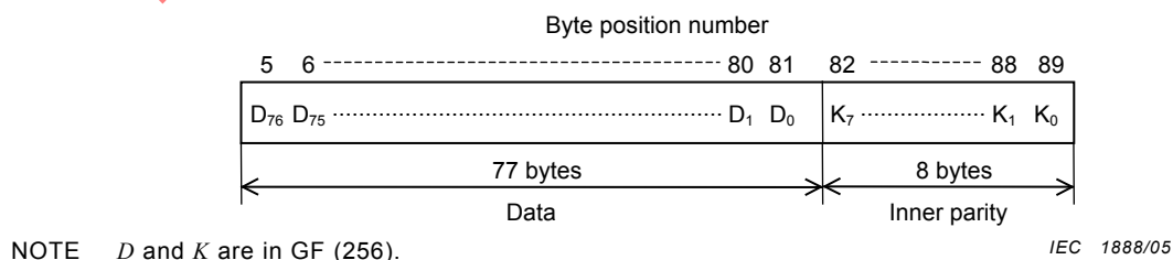
Figure 31 – Data and inner parity of a data sync block
