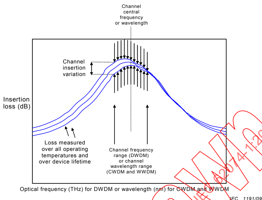
Figure 4 – Illustration of channel insertion loss variation
