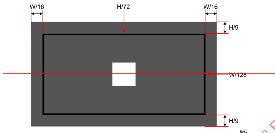
Figure 3 – Box and outline video signal, outline dimensions
