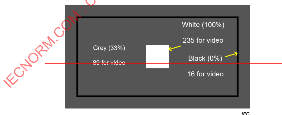
Figure 2 – Box and outline video signal, including signal drive values
