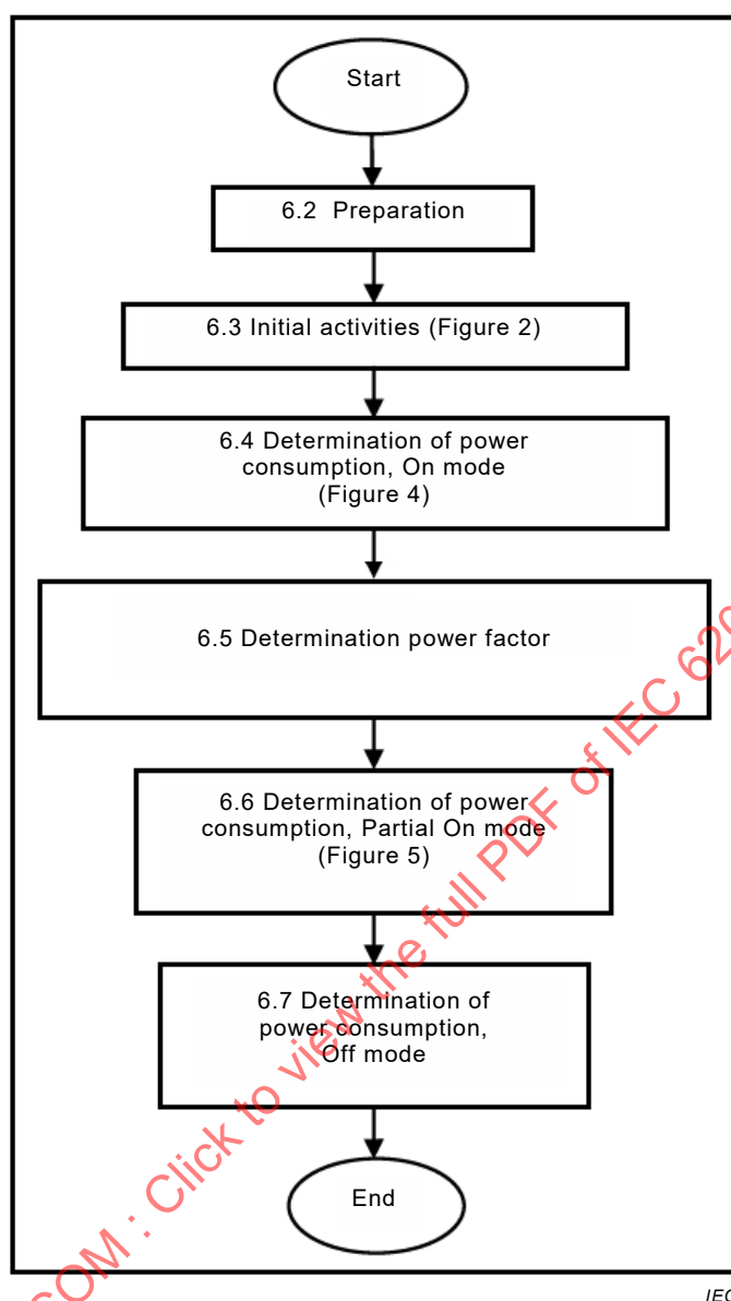
Figure 1 – Recommended order of activities
