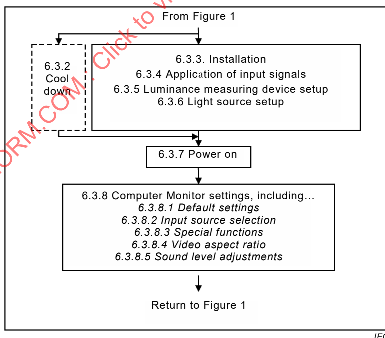
Figure 2 – Order of initial activities
