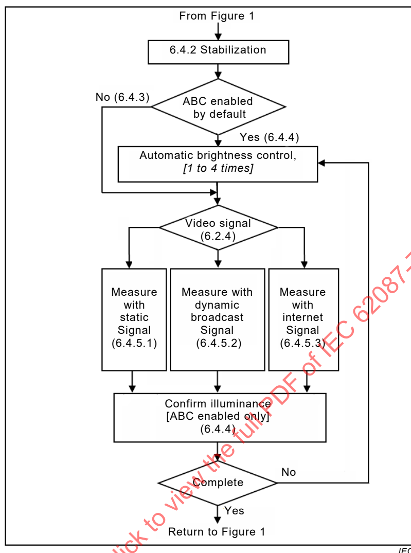
Figure 4 – Order of activities for determining power consumption, on mode
