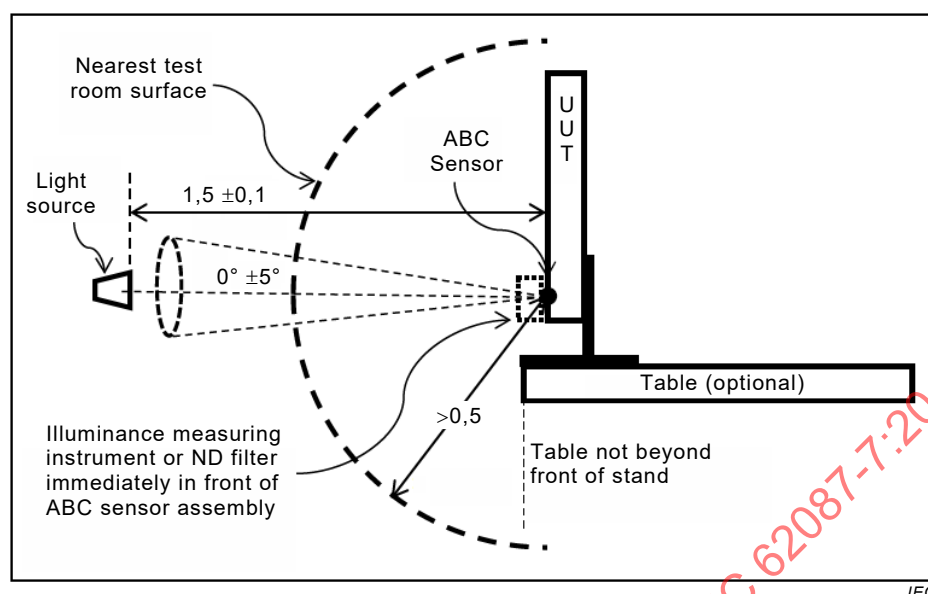
Figure 3 – Light source configuration
