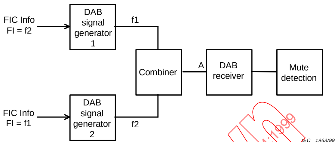
Figure 6 – Block diagram for measuring acquisition time after synchronisation loss
