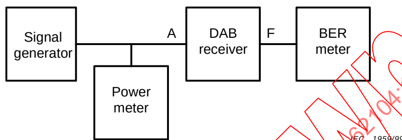
Figure 2 – Block diagram for the measurement of the sensitivity and the maximum input power
