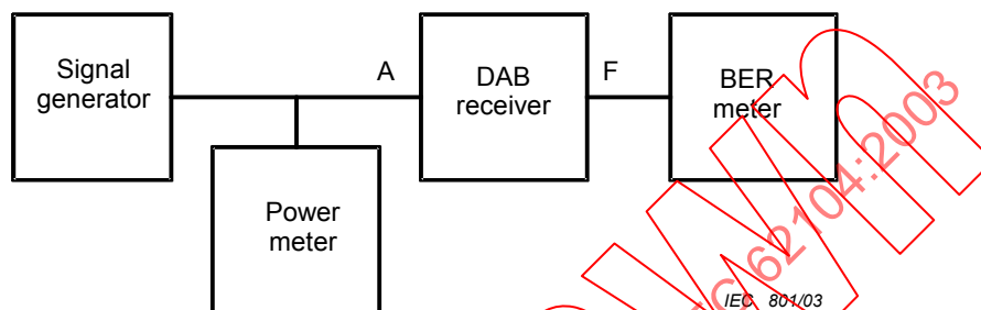
Figure 2 – Block diagram for the measurement of the sensitivity and the maximum input power
