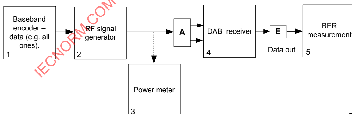
Figure 2 – Block diagram for the measurement of the sensitivity and the maximum input power, using BER
