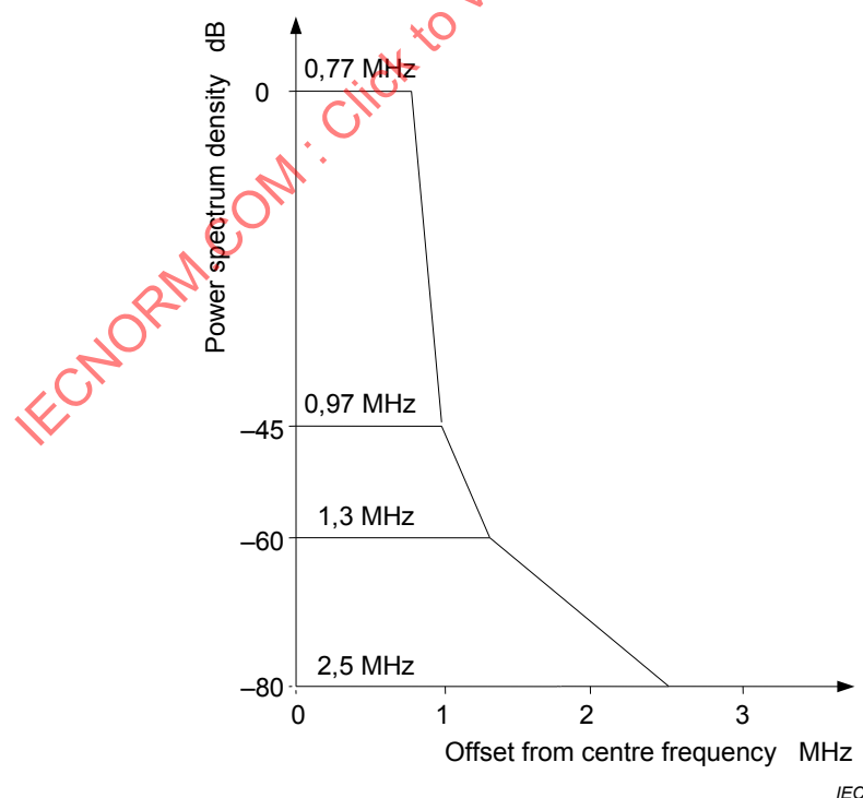
Figure 6 – Spectrum mask of the DAB signal for selectivity measurements
