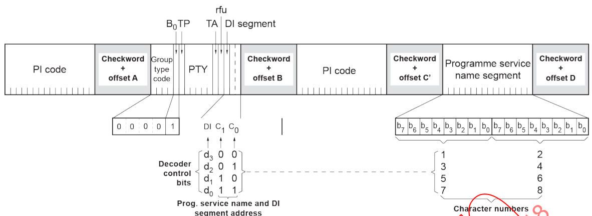
Figure 6 – Basic tuning and switching information – Group type 0B
