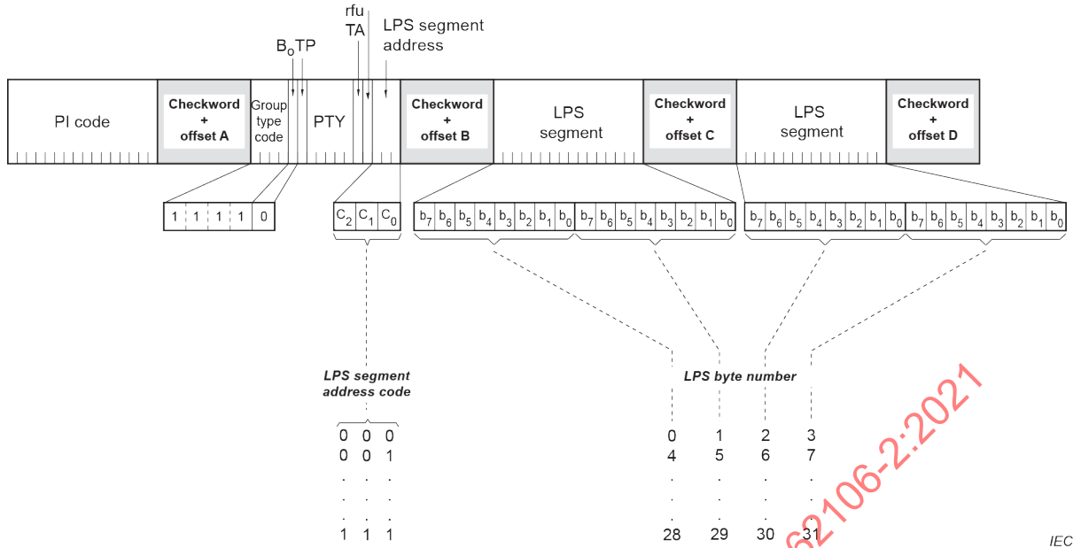
Figure 15 – Long PS, UTF-8 coded – Group type 15A
