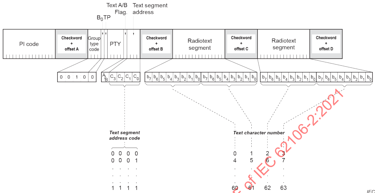
Figure 8 – RadioText – Group type 2A
