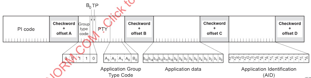
Figure 10 – Application identification for any specific ODA – Group type 3A
