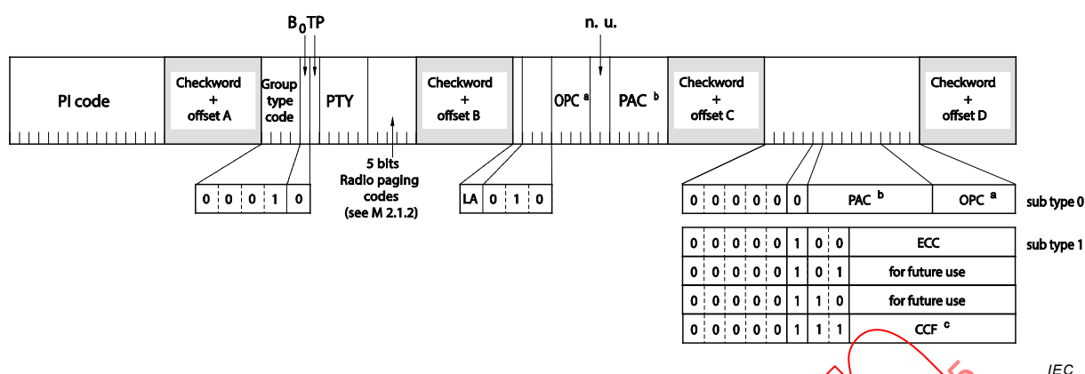
Figure M.10b – Variant 2 of 1A group without PIN
