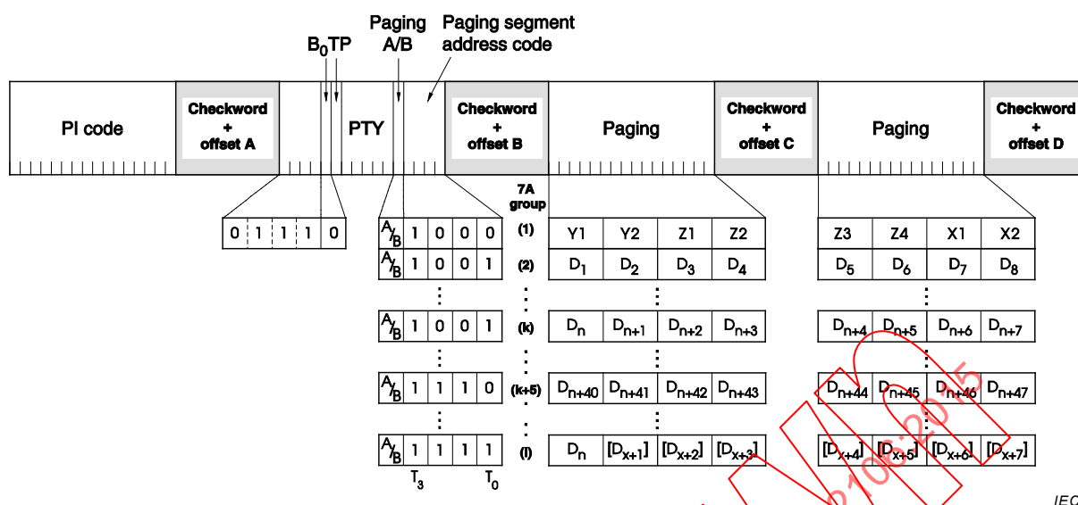
Figure M.15 – Group type 7A national paging with additional variable-length numeric message
