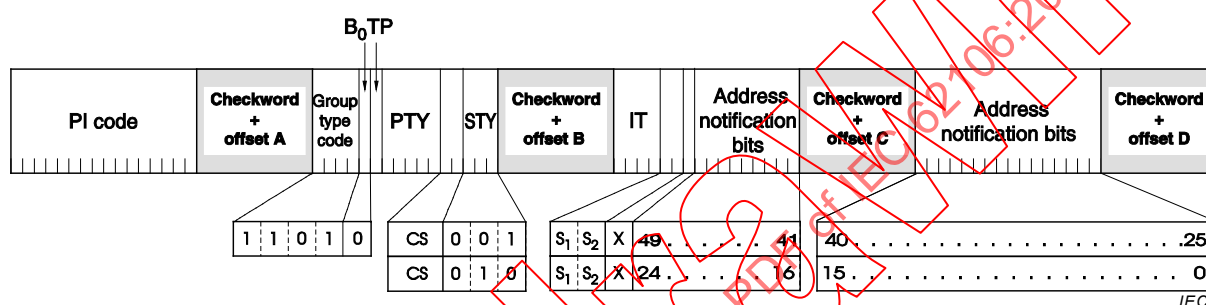
Figure M.11b – Subtype 001 and 010 – Group type 13A
