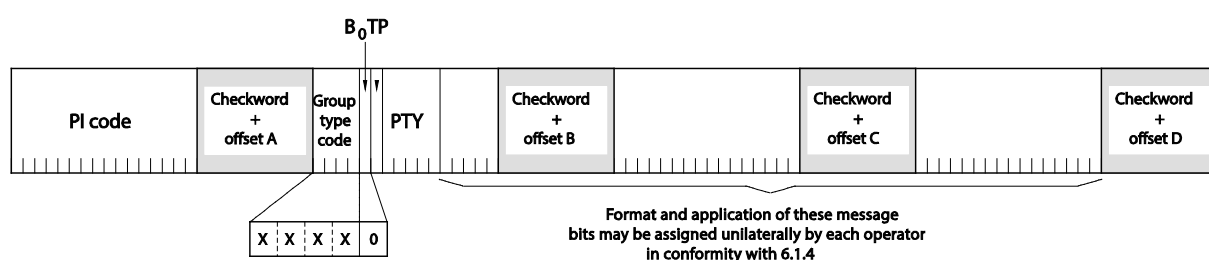
Figure 10 – ODA version A groups
