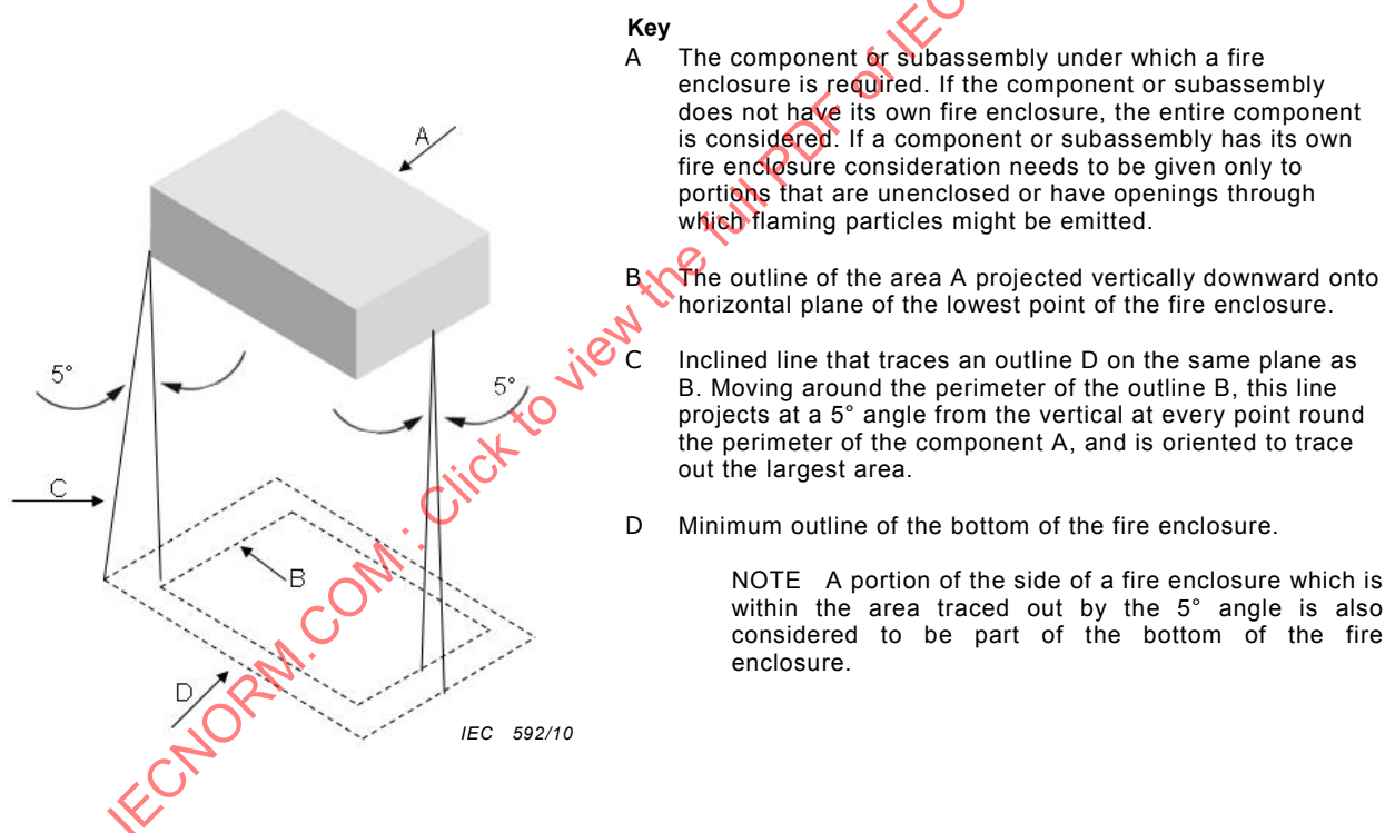
Figure 14 – Fire enclosure bottom openings below an unenclosed or partially enclosed component
