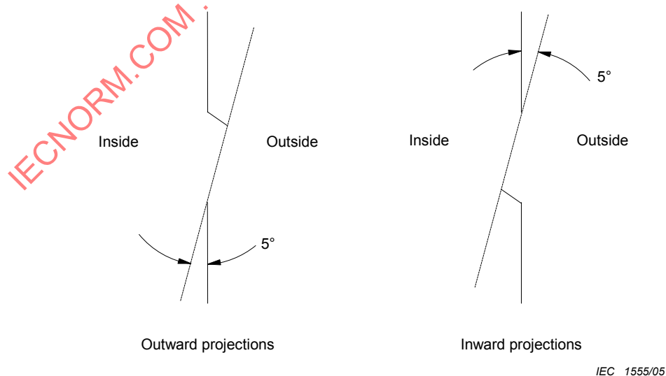
Figure 17 – Examples of louver design
