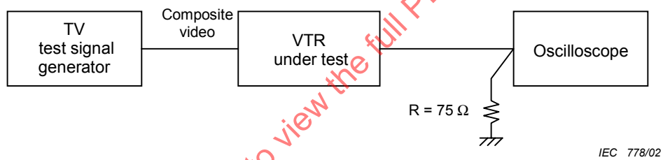
Figure 14 – Measuring block diagram for composite video signal
