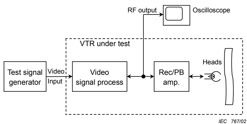
Figure 3 – Measuring block diagram for RF envelope flatness
