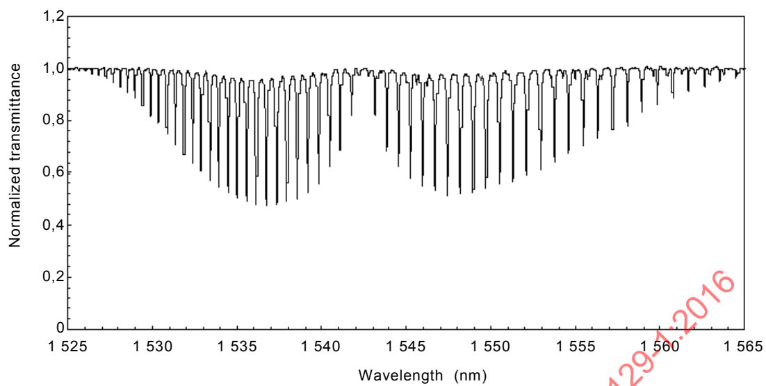
Figure D.2 – Absorption of LED light by hydrogen cyanide ( \text{H}^{13}\text{C}^{14}\text{N} )
