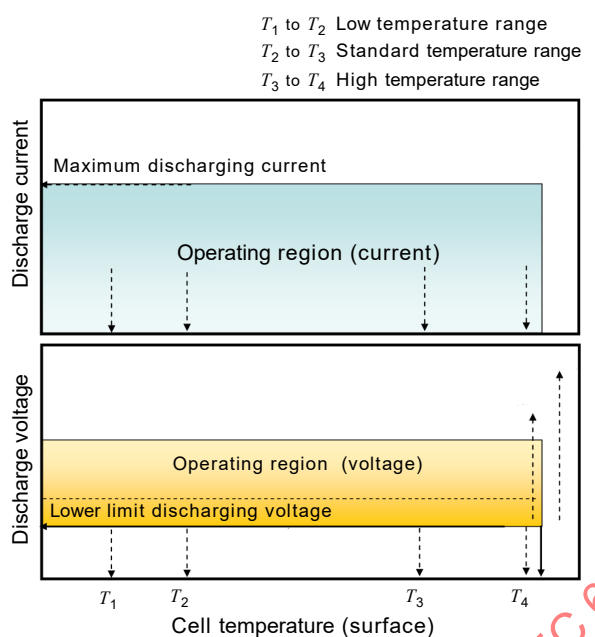
Figure A.2 – Representation of lithium ion cell operating region for discharging
