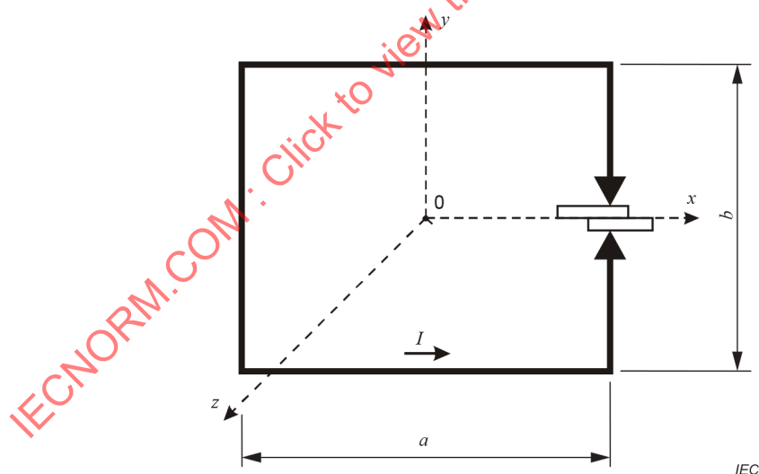
Figure 2 – Test position for H field measurement
