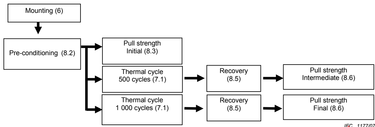
Figure 5 – Test procedure
