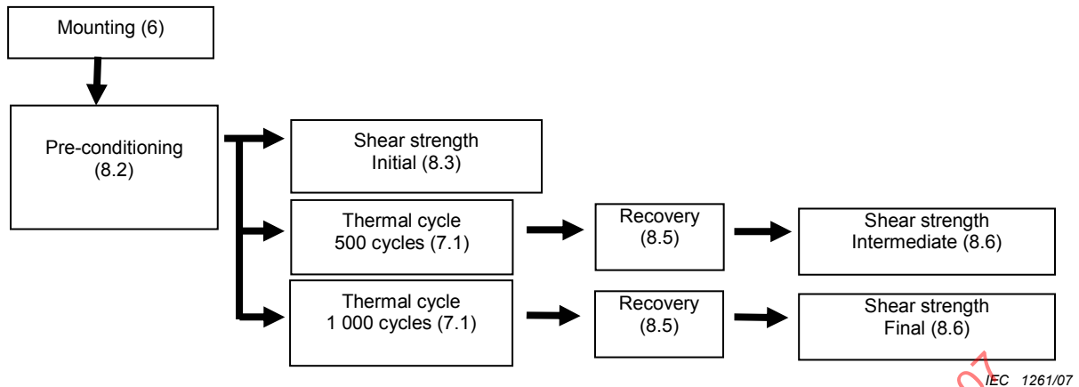
Figure 3 – Test procedure
